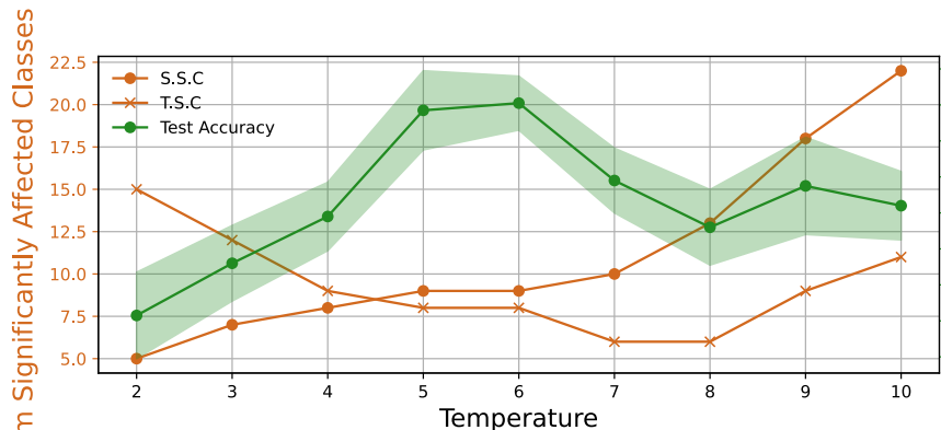
(a) CIFAR-100
